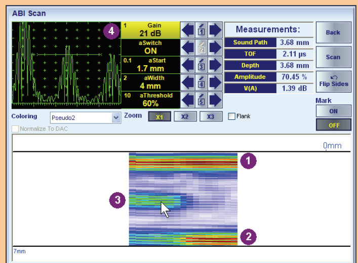
B-Scan indication of ISONIC 2010 representing inspection of composites for laminations: 1 – scanning surface; 2 – bottom surface; 3 – lamination; 4 – A-Scan corresponding to the position of cursor over image
